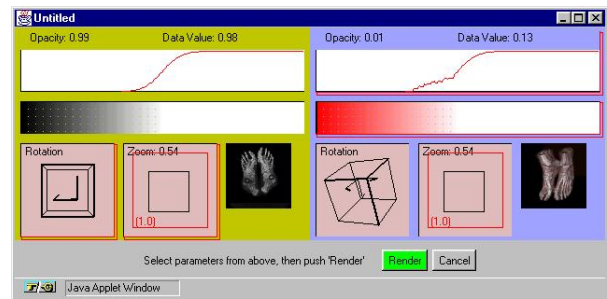
Figure 5: The interface used to combine the rendering parameters of existing graph nodes to create new nodes.
