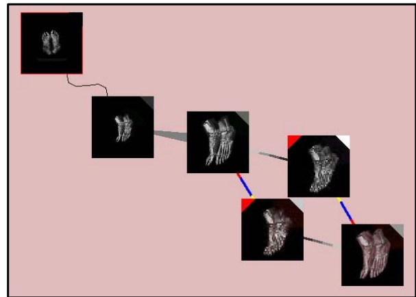
Figure 2: A small graph of some images of a foot data. The image in the top left corner is the initial image. The dataset is rotated to produce the second image. The third image is produced by zooming in on the second one. The final image comes from a change in both the color and opacity maps. The system displays this change by estimating the visual effects of both the color and opacity map changes, and rendering separate thumbnails of each. The red mark in the corner of these images indicates that they are thumbnails. The user can click on a thumbnail to render a full size image with the rendering parameters of that graph node. Note that the intermediate images are rendered at low resolution to minimize rendering time.
